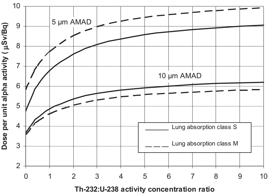
FIG. 4. Dose coefficients for gross alpha activity, assuming 75% retention of radon and thoron on a sampling filter.
