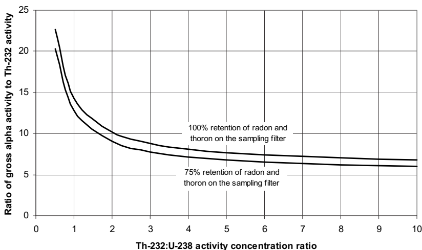
FIG. 3. Relationship between gross alpha activity and ^{232}\text{Th} activity in dust particles captured on a sampling filter.
