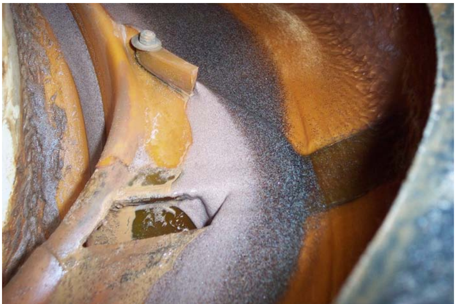
FIG. 12. Detailed view of a spiral used in the primary separation process.
